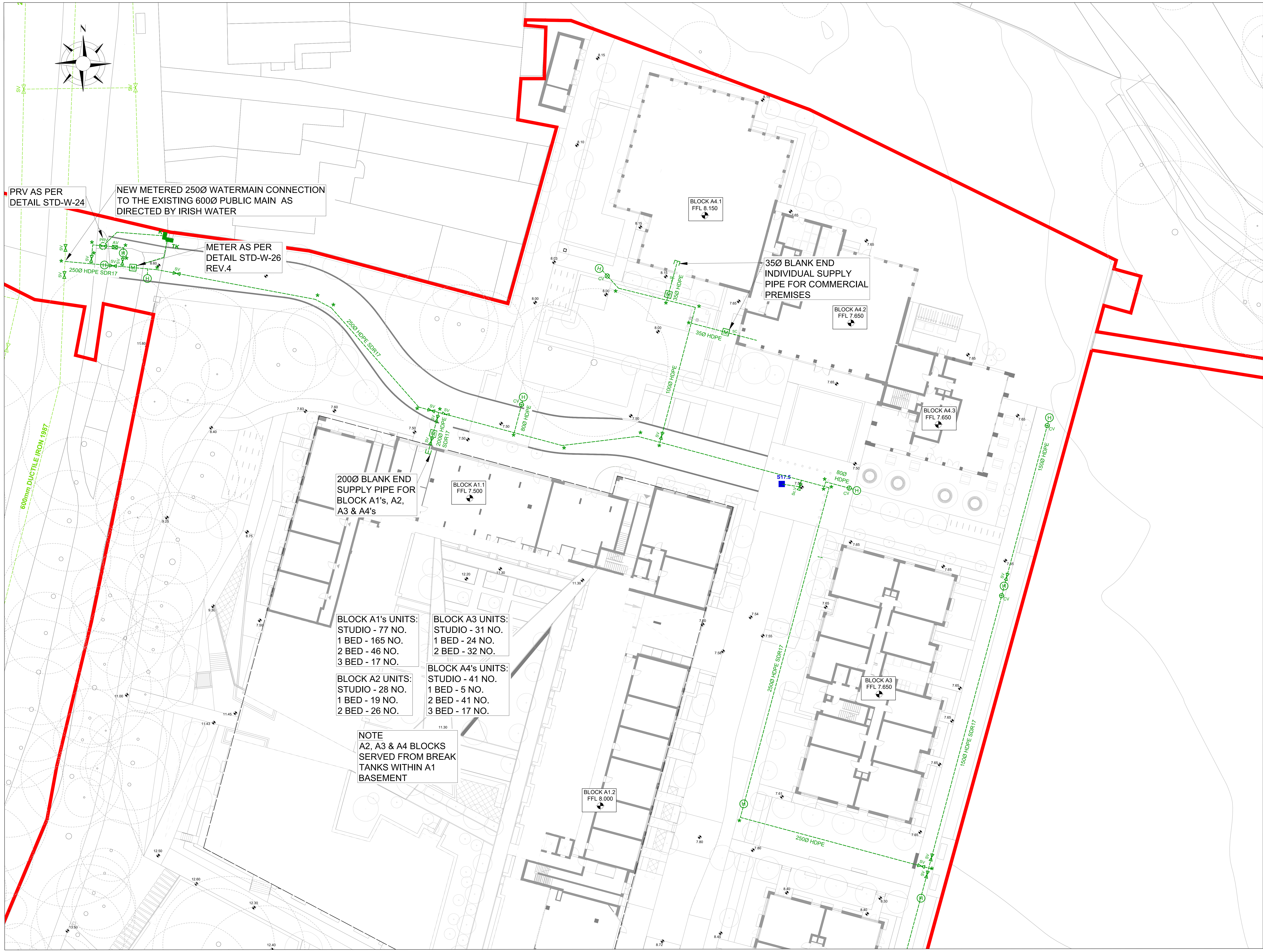
PROPOSED WATERMAIN SITE PLAN LAYOUT - SHEET 1 OF 8 SCALE @ A0: 1:200 SCALE @ A2: 1:400
